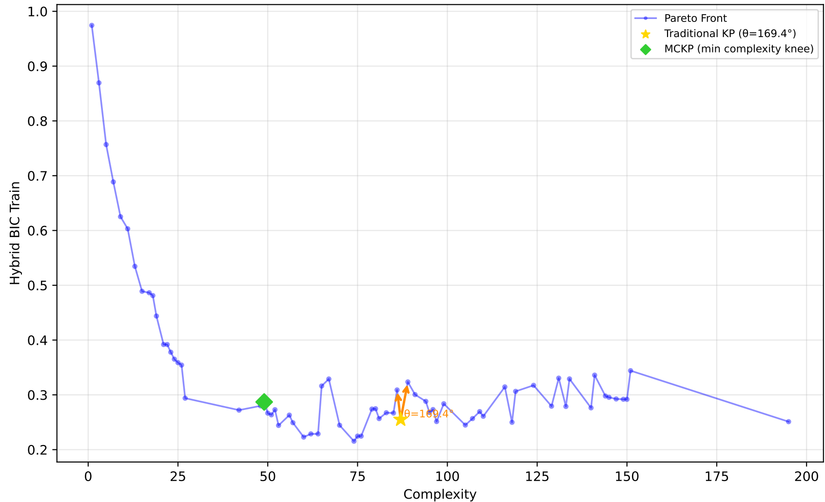
229_pwLinear - Run 18 - MVP - Hybrid BIC Train \lambda_1=0.50, \lambda_2=0.00, \lambda_3=0.00 | Difficulty: 0.95 | Method: hmr
