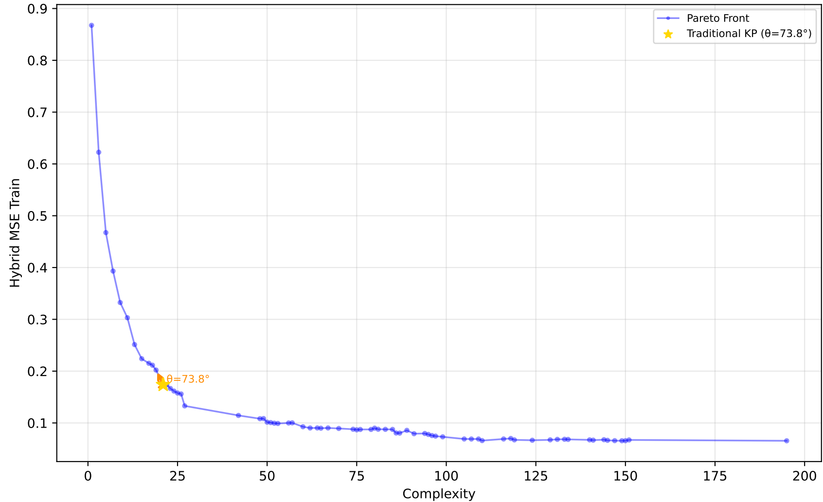
229_pwLinear - Run 18 - MVP - Hybrid MSE Train \lambda_1=0.50, \lambda_2=0.00, \lambda_3=0.00 | Difficulty: 0.95 | Method: hmr
