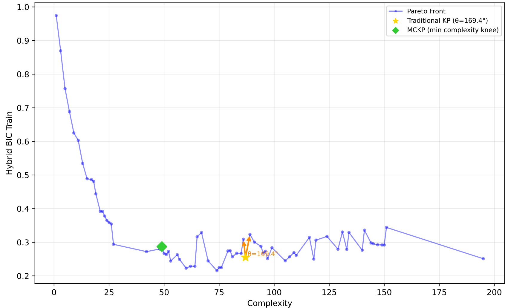
229_pwLinear - Run 18 - SVP - Hybrid BIC Train \lambda_1=0.50, \lambda_2=0.00, \lambda_3=0.00 | Difficulty: 0.95 | Method: hmr
