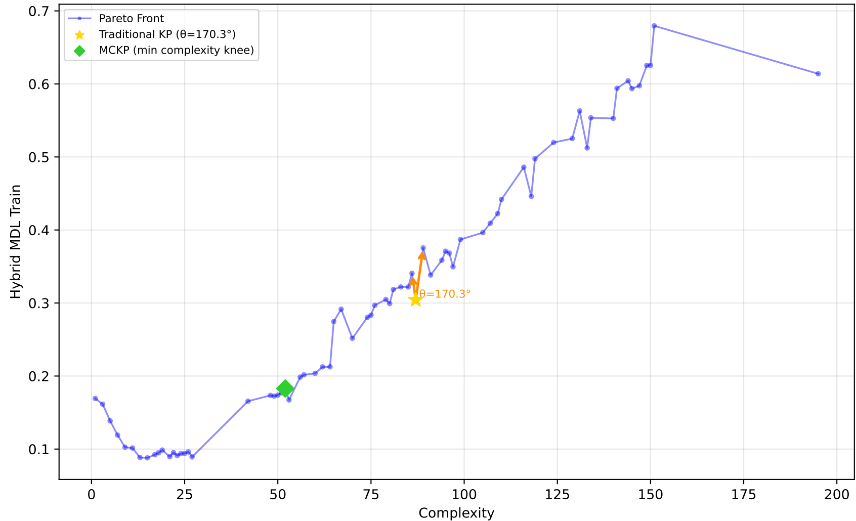
229_pwLinear - Run 18 - SVP - Hybrid MDL Train \lambda_1=0.50, \lambda_2=0.00, \lambda_3=0.00 | Difficulty: 0.95 | Method: hmr
