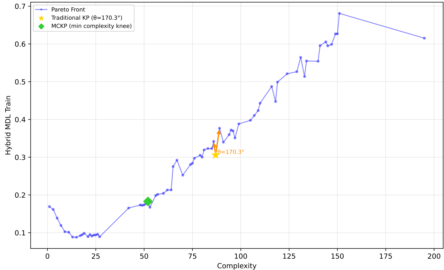
229_pwLinear - Run 18 - SVP - Hybrid MDL Train \lambda_1=0.50, \lambda_2=0.10, \lambda_3=0.00 | Difficulty: 0.95 | Method: hmr
