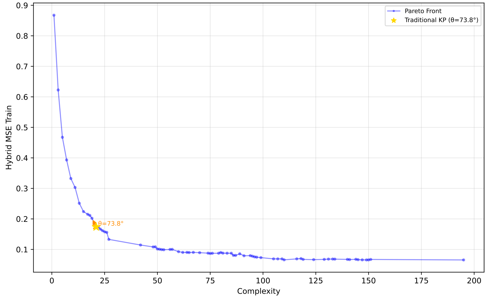
229_pwLinear - Run 18 - SVP - Hybrid MSE Train \lambda_1=0.50, \lambda_2=0.00, \lambda_3=0.00 | Difficulty: 0.95 | Method: hmr
