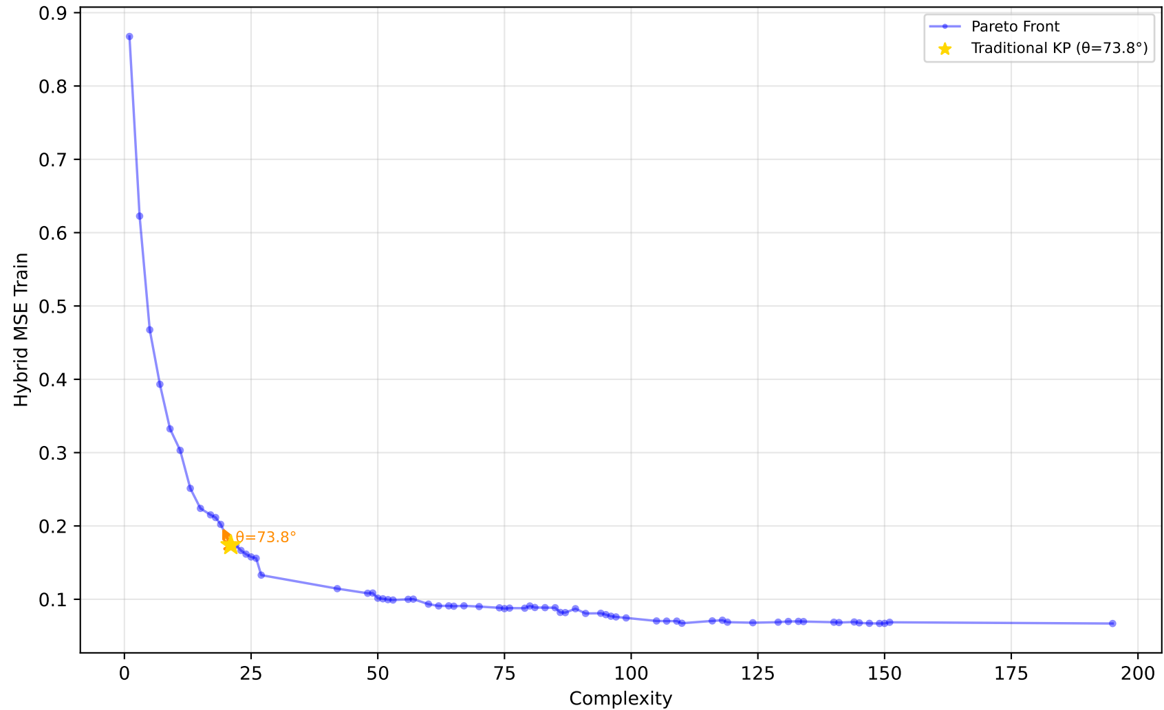
229_pwLinear - Run 18 - SVP - Hybrid MSE Train \lambda_1=0.50, \lambda_2=0.10, \lambda_3=0.00 | Difficulty: 0.95 | Method: hmr
