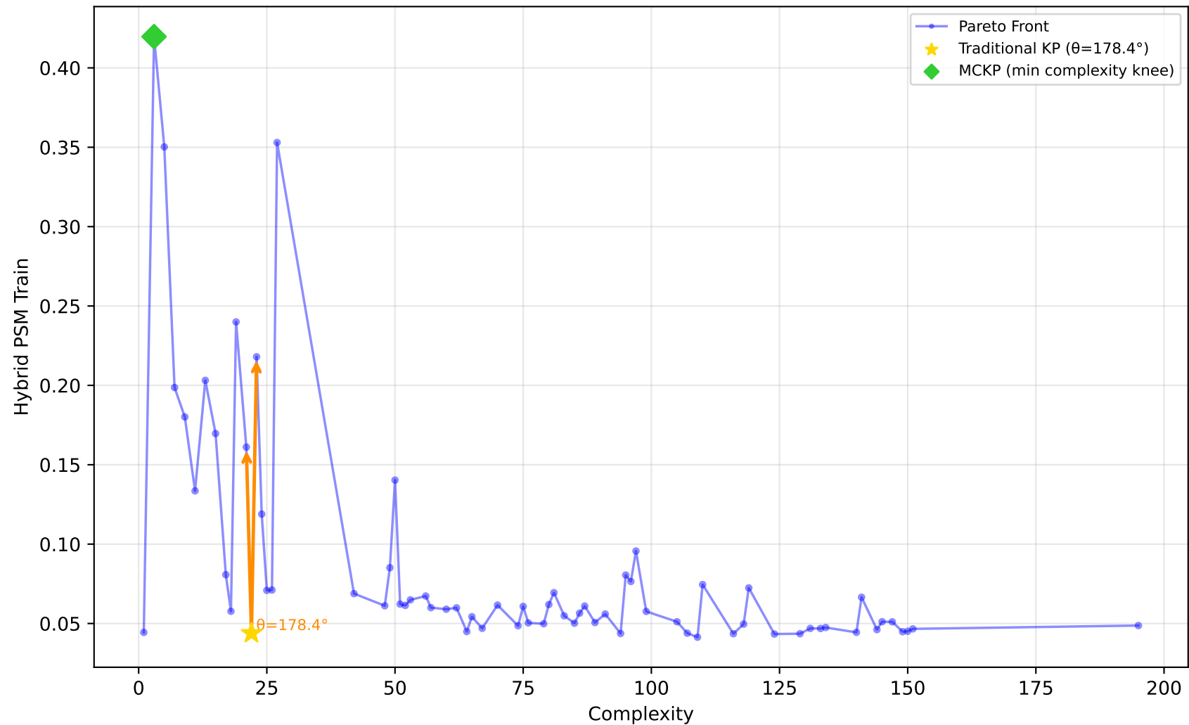
229_pwLinear - Run 18 - SVP - Hybrid PSM Train \lambda_1=0.50, \bar{\lambda}_2=0.10, \lambda_3=0.00 | Difficulty: 0.95 | Method: hmr
