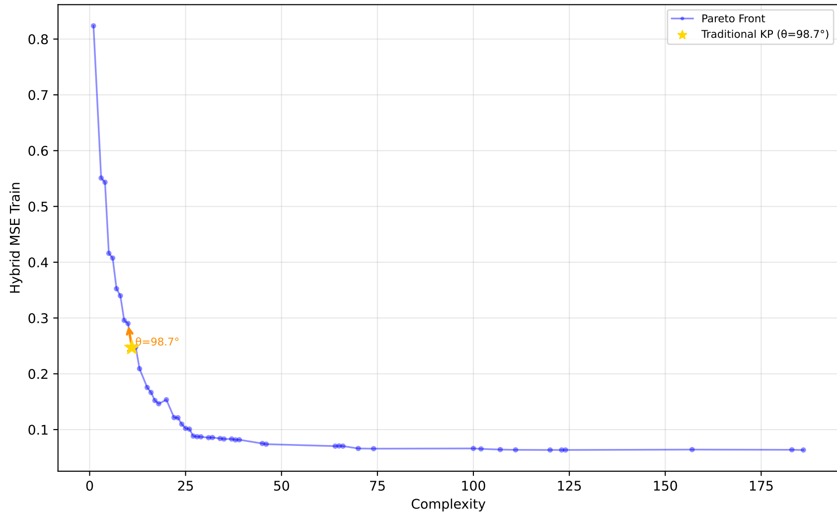
229_pwLinear - Run 19 - MVP - Hybrid MSE Train \lambda_1=0.50, \lambda_2=0.00, \lambda_3=0.00 | Difficulty: 1.00 | Method: hmr
