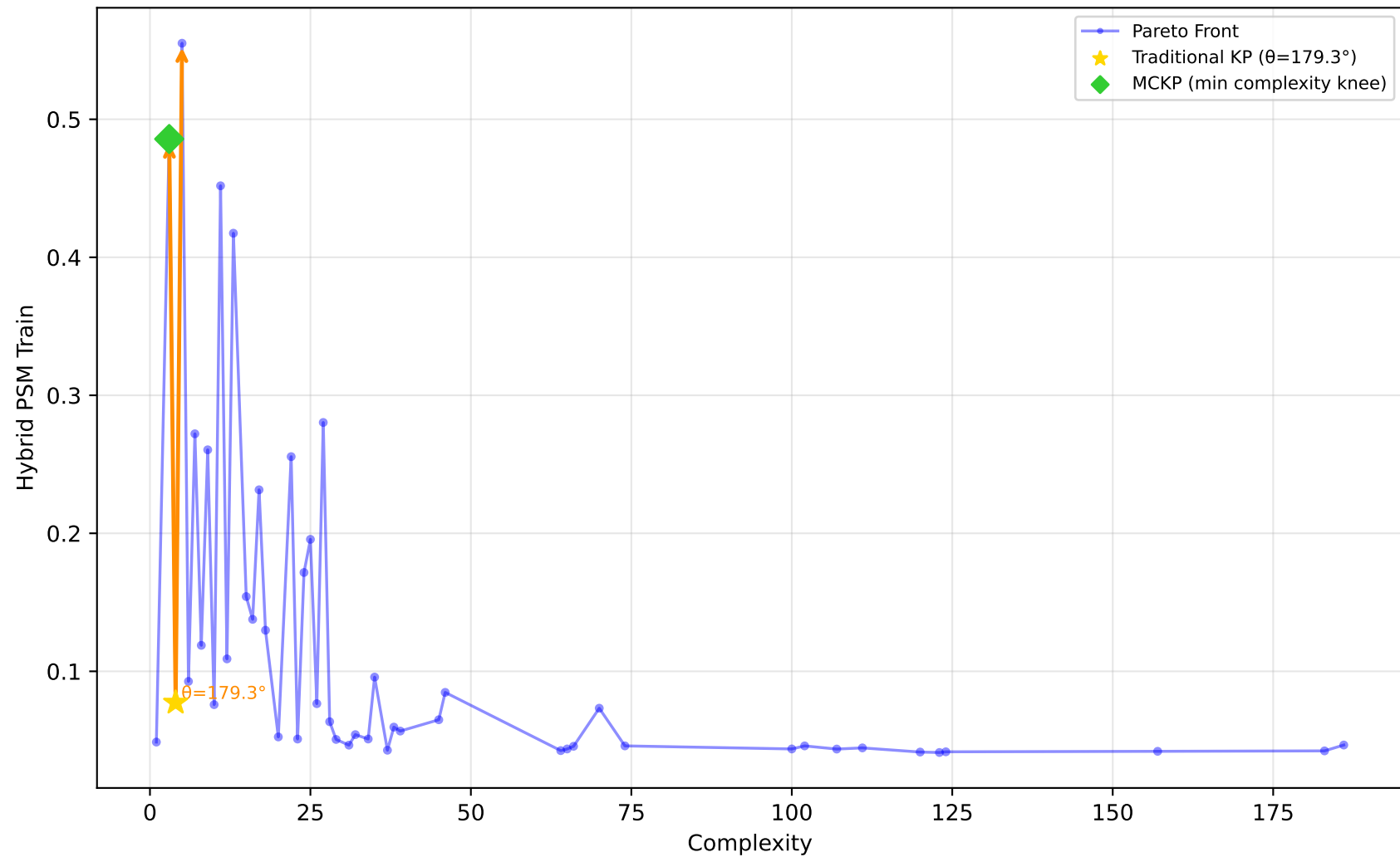
229_pwLinear - Run 19 - MVP - Hybrid PSM Train \lambda_1=0.50, \lambda_2=0.00, \lambda_3=0.00 | Difficulty: 1.00 | Method: hmr
