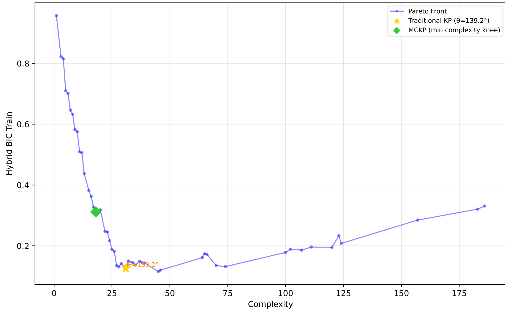
229_pwLinear - Run 19 - SVP - Hybrid BIC Train \lambda_1=0.50, \lambda_2=0.00, \lambda_3=0.00 | Difficulty: 1.00 | Method: hmr
