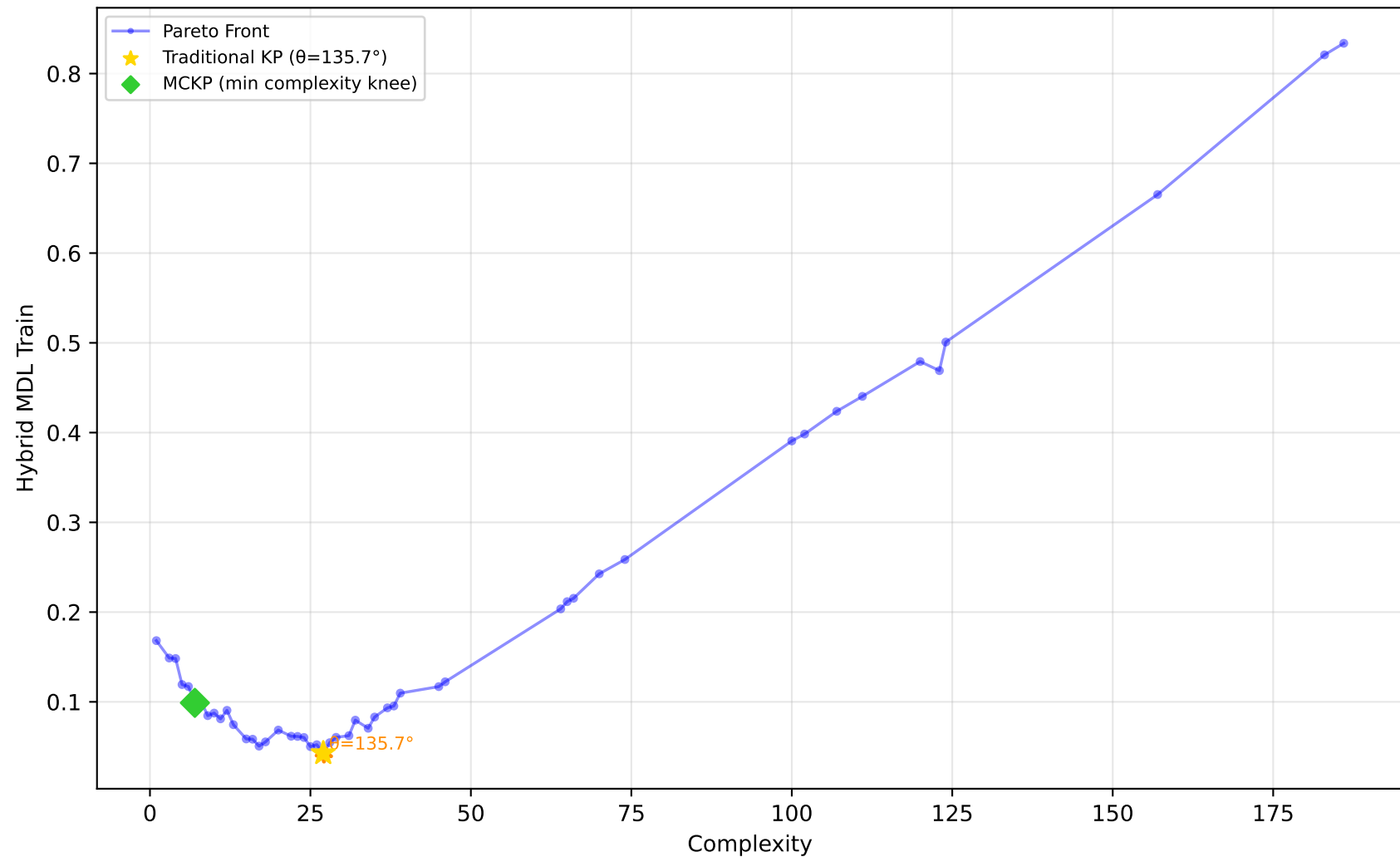
229_pwLinear - Run 19 - SVP - Hybrid MDL Train \lambda_1=0.50, \lambda_2=0.00, \lambda_3=0.00 | Difficulty: 1.00 | Method: hmr
