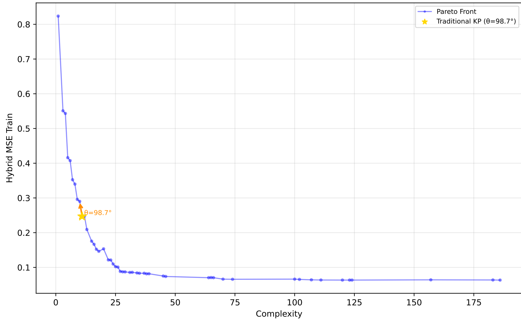
229_pwLinear - Run 19 - SVP - Hybrid MSE Train \lambda_1=0.50, \lambda_2=0.00, \lambda_3=0.00 | Difficulty: 1.00 | Method: hmr
