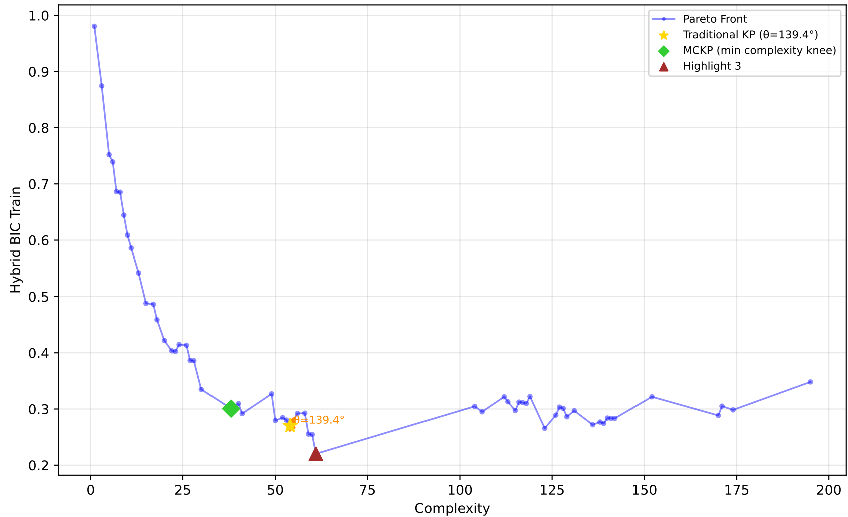
229_pwLinear - Run 1 - SVP - Hybrid BIC Train \lambda_1=0.50, \lambda_2=0.00, \lambda_3=0.00 | Difficulty: 1.00 | Method: hmr
