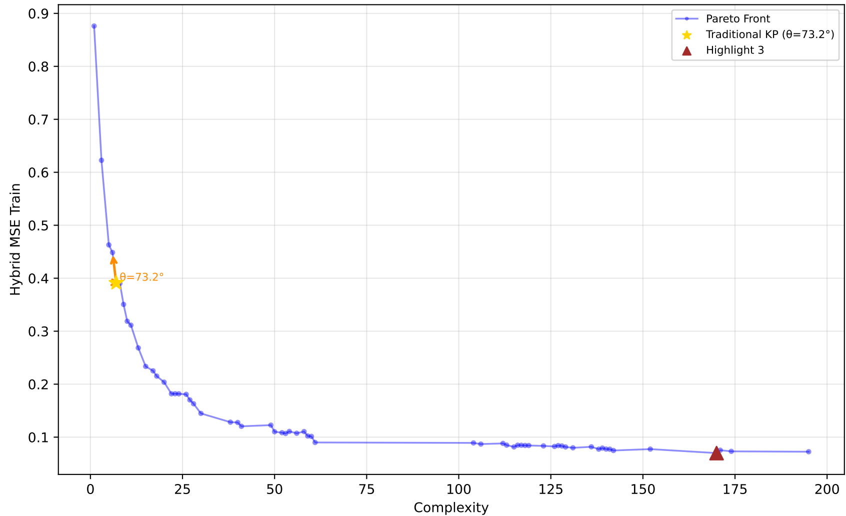
229_pwLinear - Run 1 - SVP - Hybrid MSE Train \lambda_1=0.50, \lambda_2=0.00, \lambda_3=0.00 | Difficulty: 1.00 | Method: hmr
