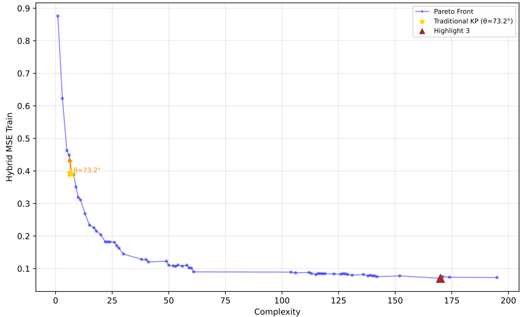
229_pwLinear - Run 1 - SVP - Hybrid MSE Train \lambda_1=0.50, \lambda_2=0.10, \lambda_3=0.00 | Difficulty: 1.00 | Method: hmr
