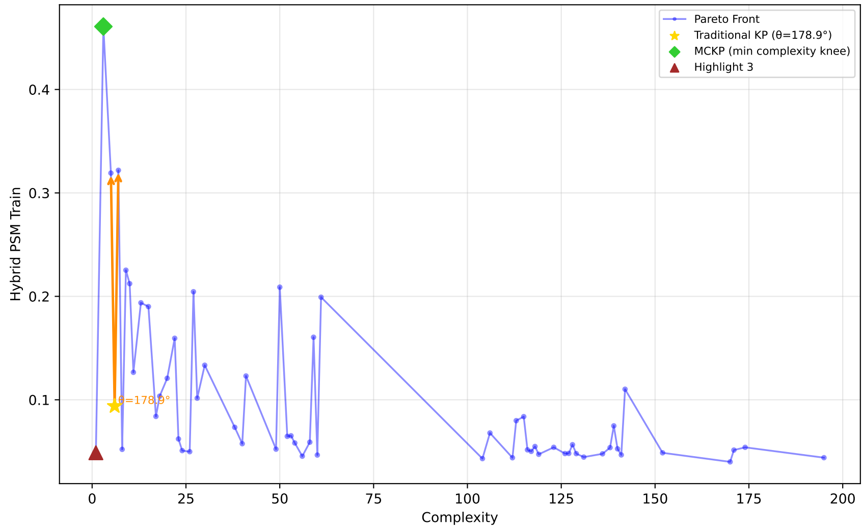
229_pwLinear - Run 1 - SVP - Hybrid PSM Train \lambda_1=0.50, \lambda_2=0.00, \lambda_3=0.00 | Difficulty: 1.00 | Method: hmr
