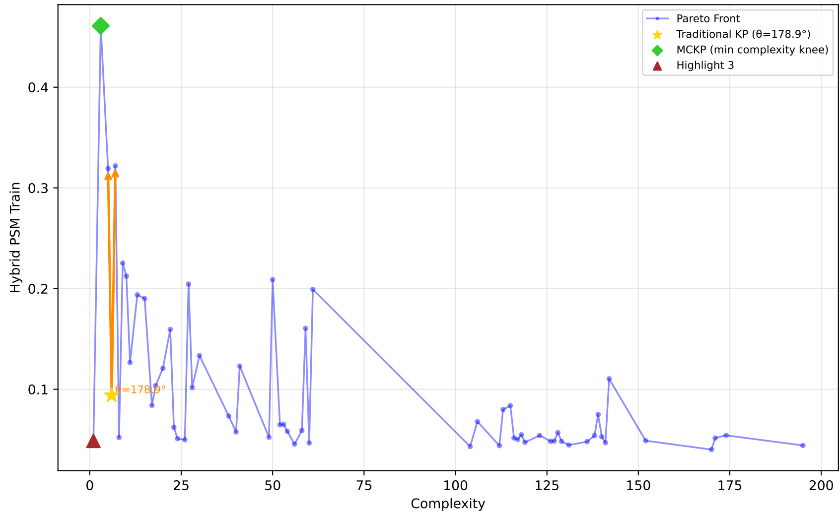
229_pwLinear - Run 1 - SVP - Hybrid PSM Train \lambda_1=0.50, \lambda_2=0.10, \lambda_3=0.00 | Difficulty: 1.00 | Method: hmr
