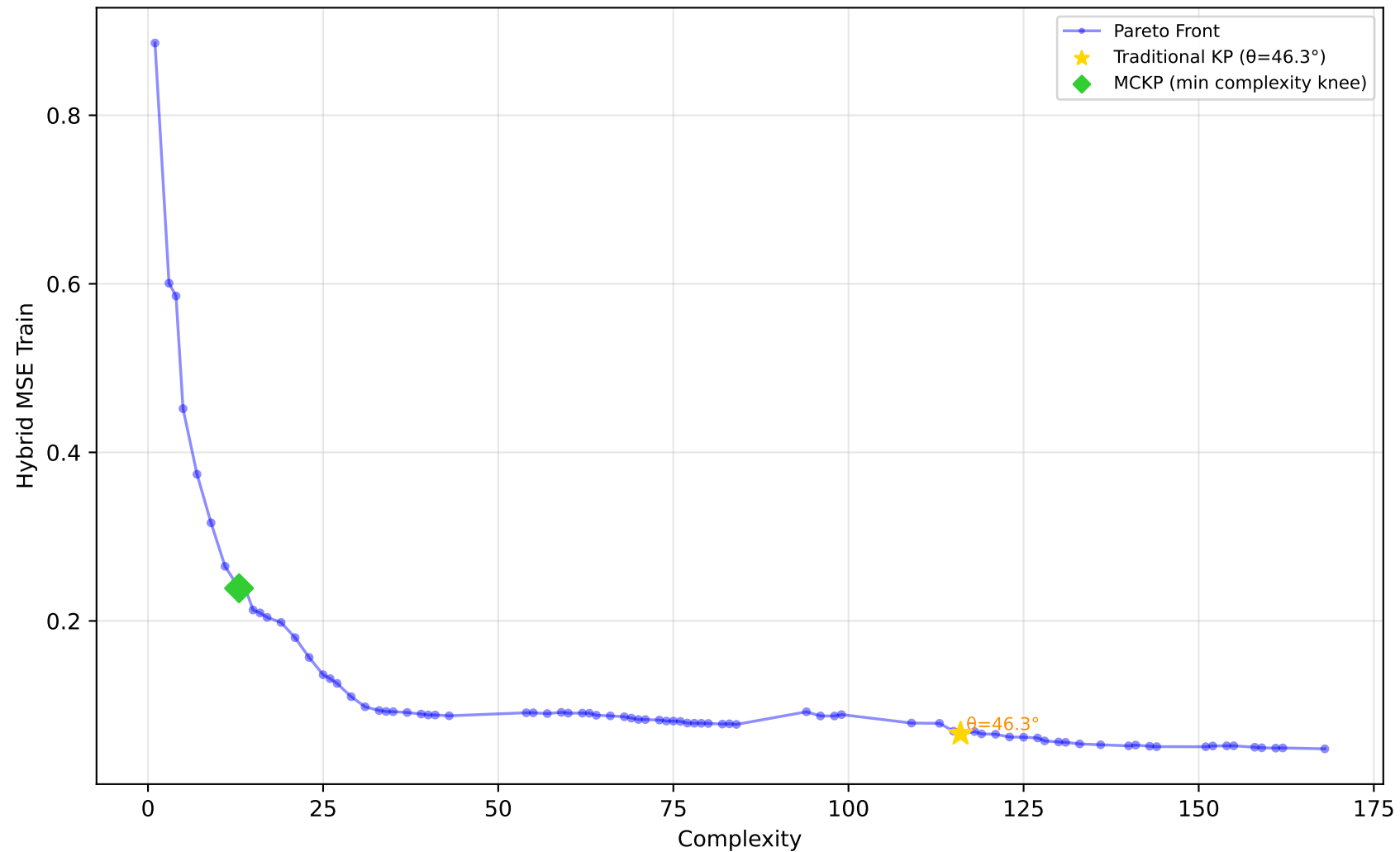
229_pwLinear - Run 20 - MVP - Hybrid MSE Train \lambda_1=0.50, \lambda_2=0.00, \lambda_3=0.00 | Difficulty: 0.90 | Method: hmr
