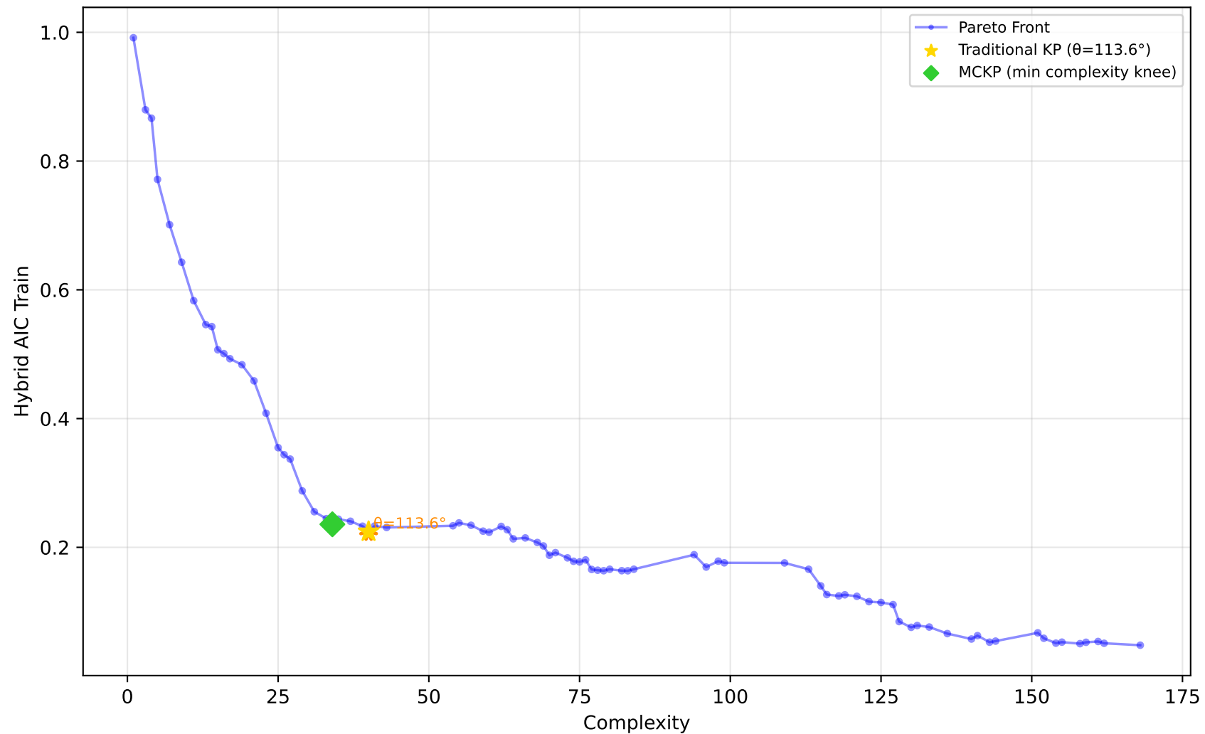
229_pwLinear - Run 20 - SVP - Hybrid AIC Train \lambda_1=0.50, \bar{\lambda}_2=0.00, \lambda_3=0.00 | Difficulty: 0.90 | Method: hmr
