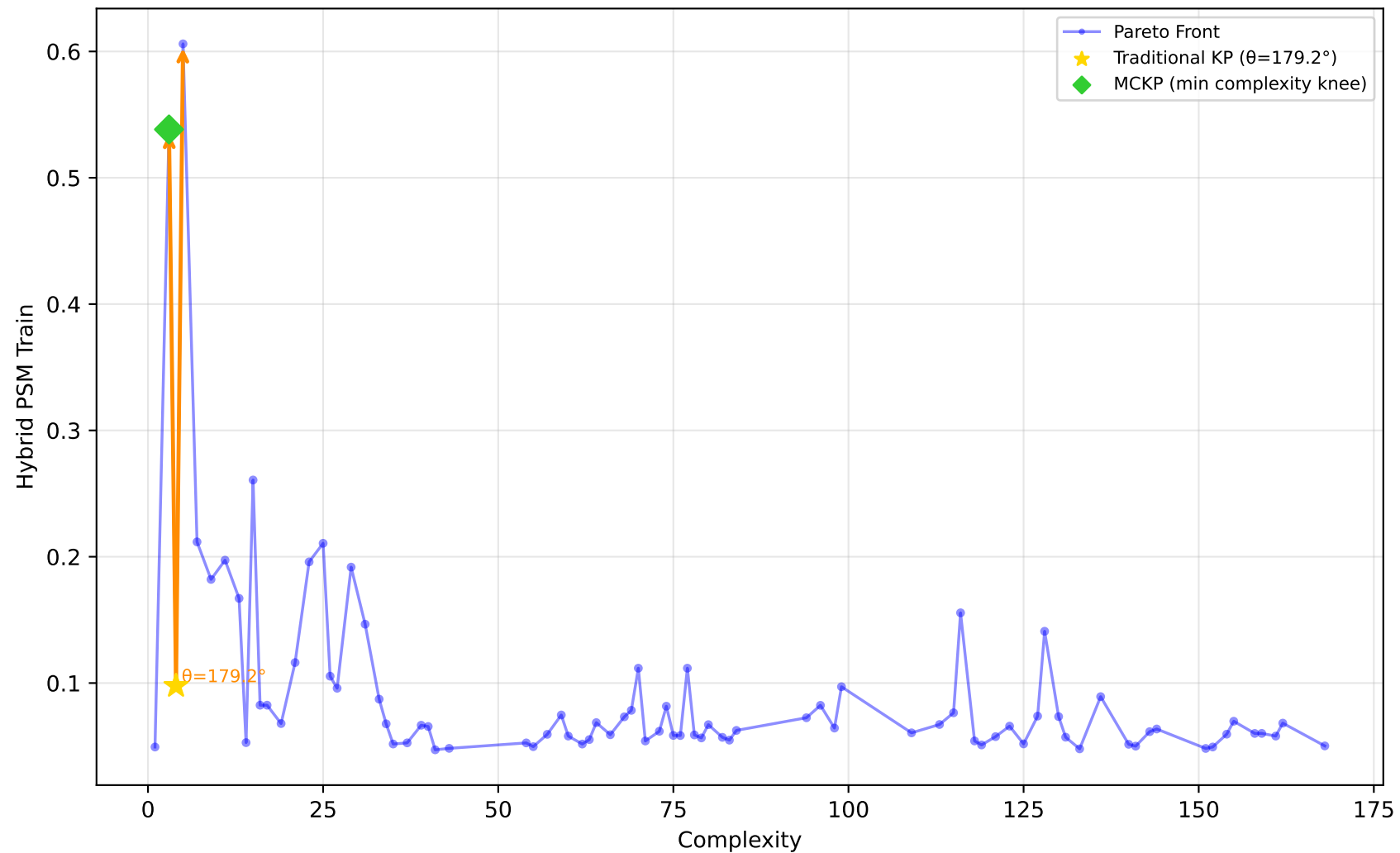
229_pwLinear - Run 20 - SVP - Hybrid PSM Train \lambda_1=0.50, \bar{\lambda}_2=0.10, \lambda_3=0.00 | Difficulty: 0.90 | Method: hmr
