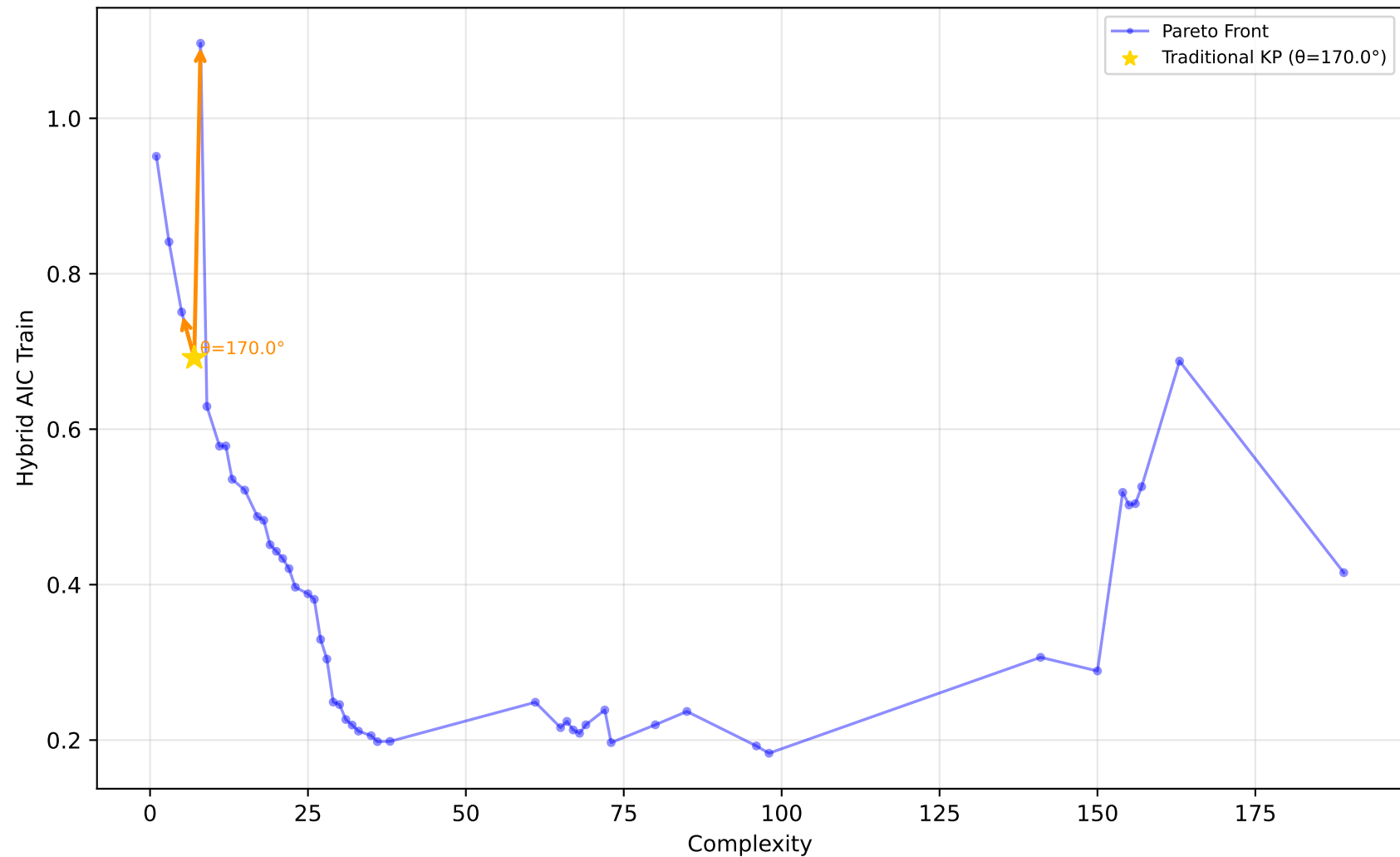
229_pwLinear - Run 21 - SVP - Hybrid AIC Train \lambda_1=0.50, \lambda_2=0.10, \lambda_3=0.00 | Difficulty: 1.00 | Method: hmr
