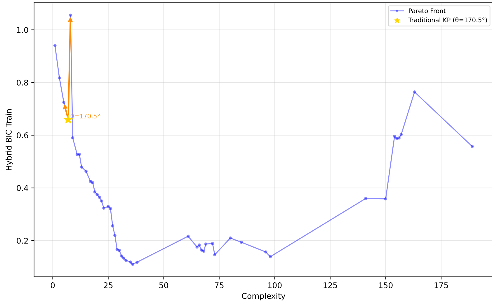
229_pwLinear - Run 21 - SVP - Hybrid BIC Train \lambda_1=0.50, \lambda_2=0.10, \lambda_3=0.00 | Difficulty: 1.00 | Method: hmr
