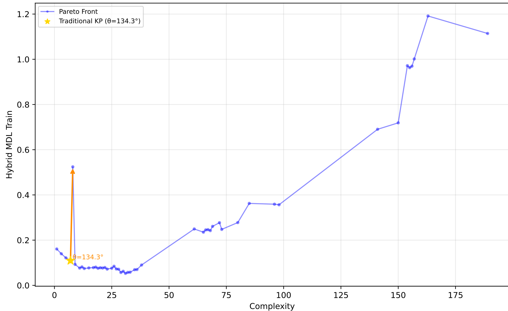
229_pwLinear - Run 21 - SVP - Hybrid MDL Train \lambda_1=0.50, \lambda_2=0.10, \lambda_3=0.00 | Difficulty: 1.00 | Method: hmr
