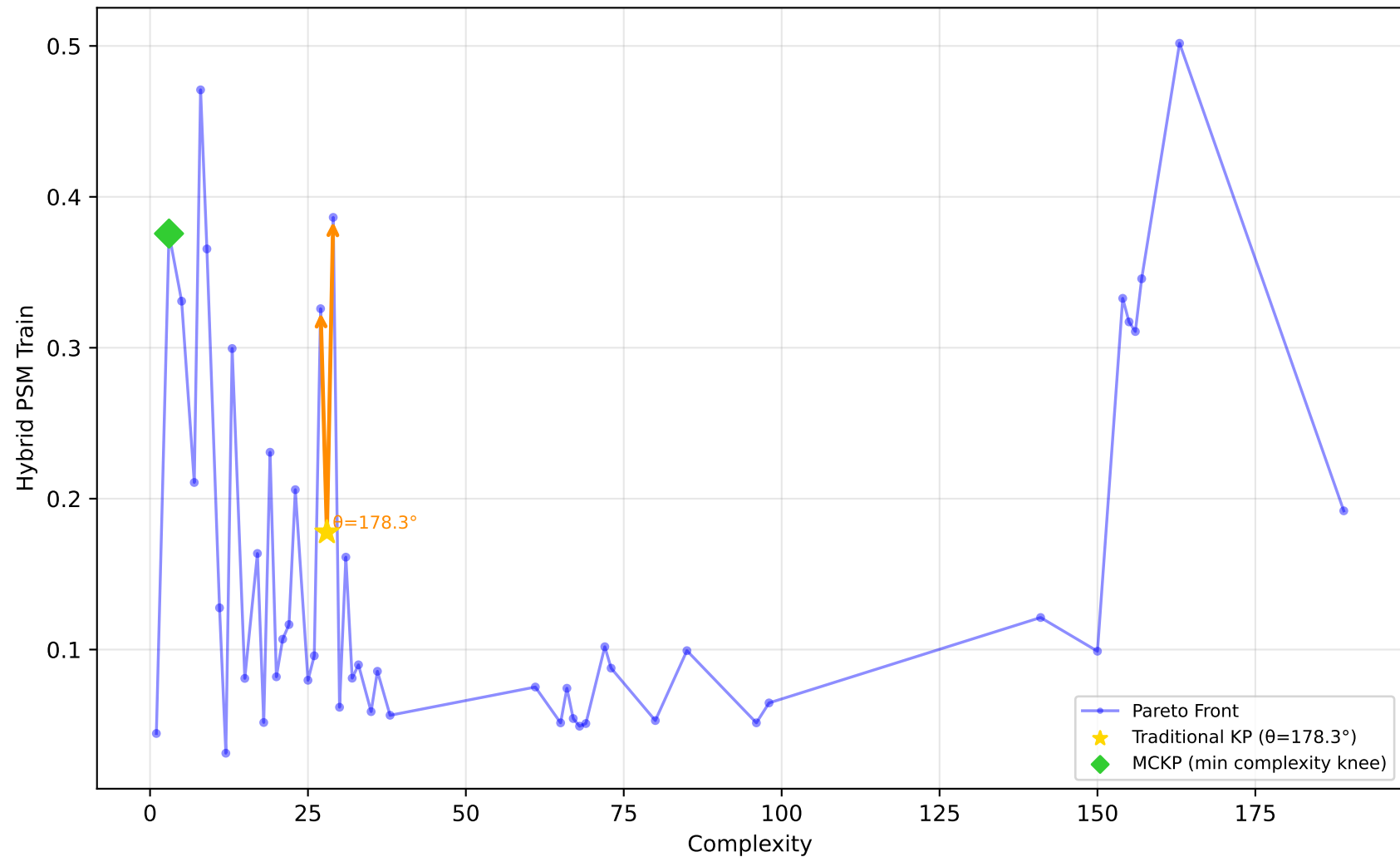
229_pwLinear - Run 21 - SVP - Hybrid PSM Train \lambda_1=0.50, \lambda_2=0.10, \lambda_3=0.00 | Difficulty: 1.00 | Method: hmr
