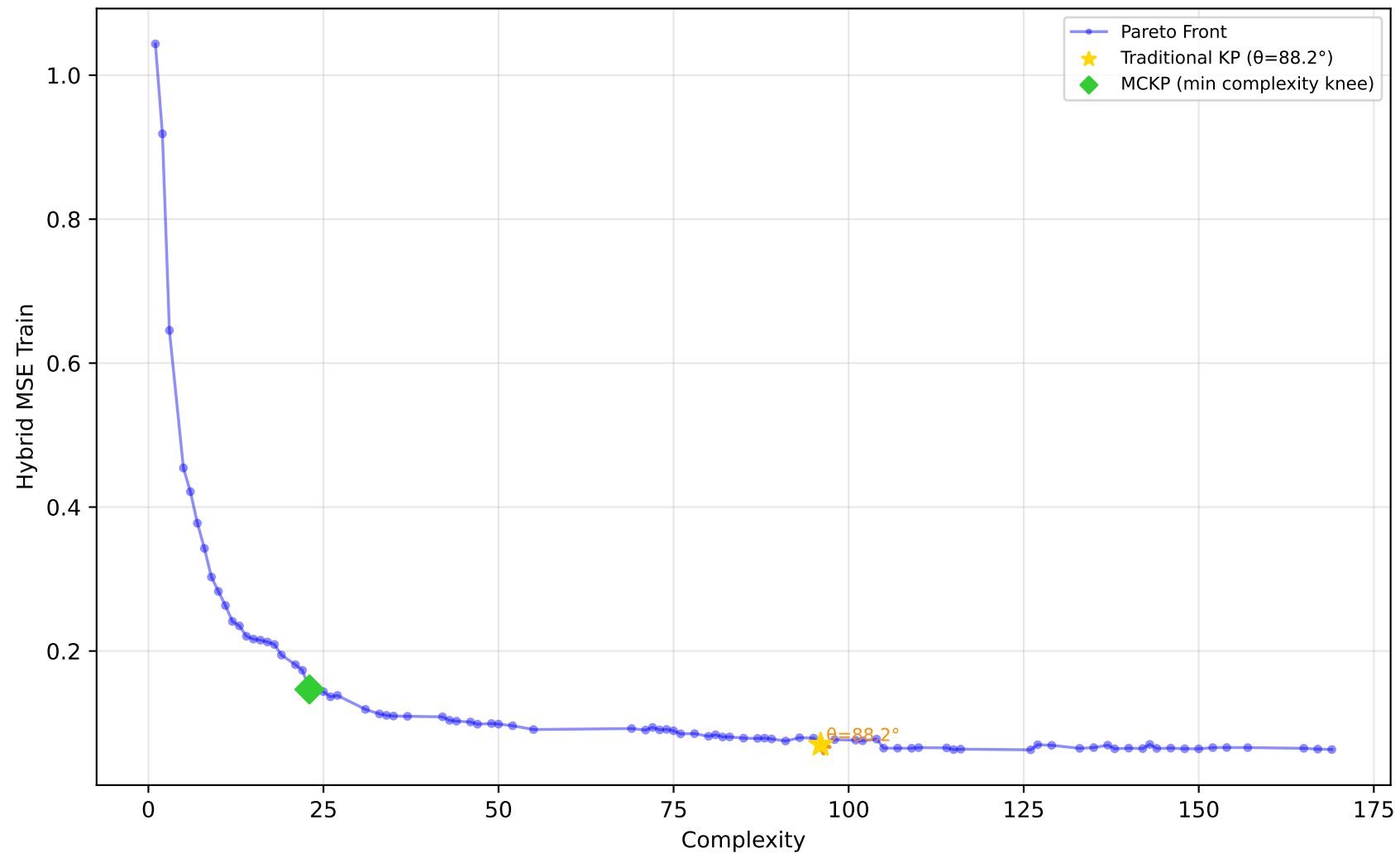
229_pwLinear - Run 22 - MVP - Hybrid MSE Train \lambda_1=0.50 , \lambda_2=0.00 , \lambda_3=0.00 | Difficulty: 1.00 | Method: hmr
