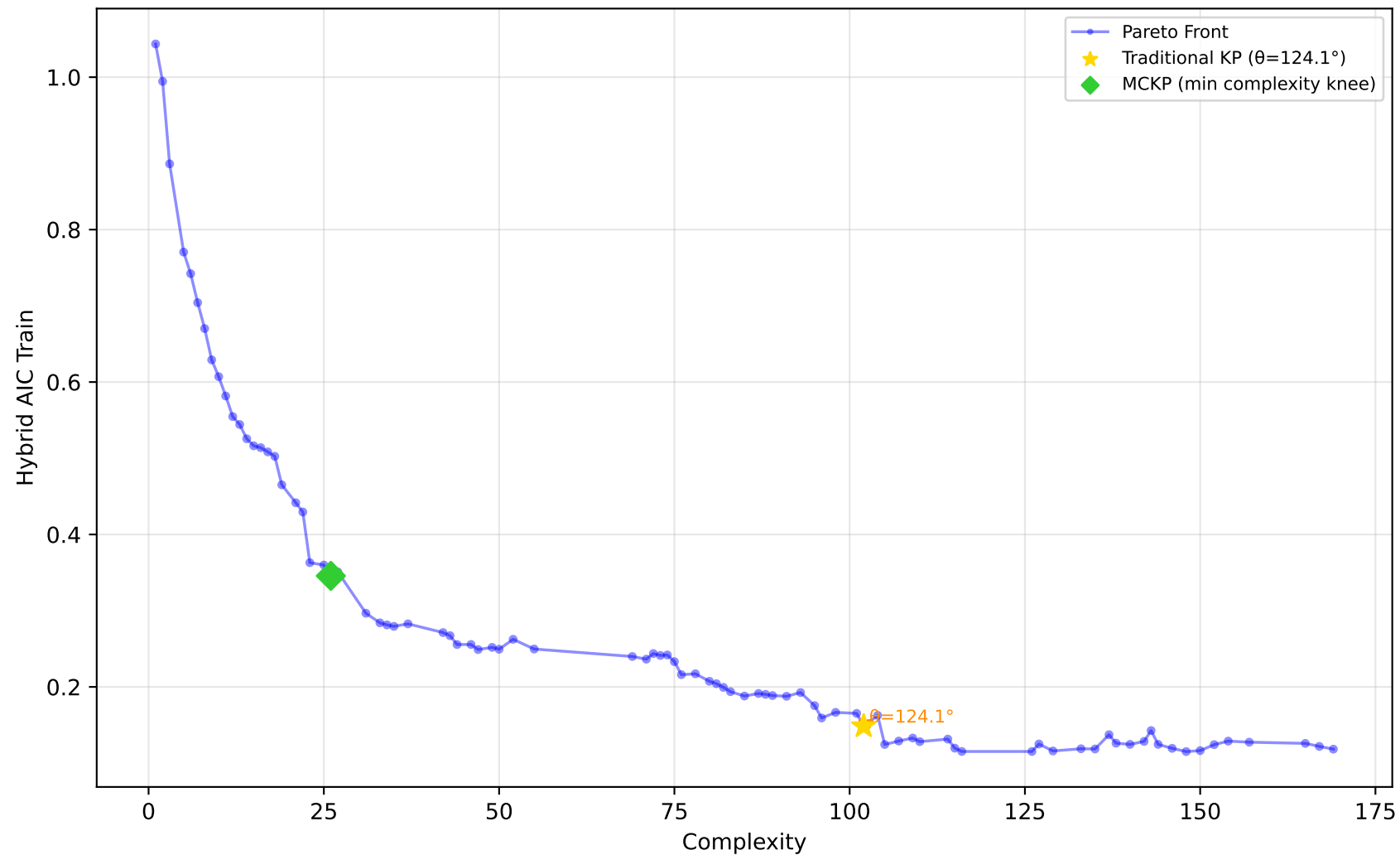
229_pwLinear - Run 22 - SVP - Hybrid AIC Train \lambda_1=0.50, \lambda_2=0.00, \lambda_3=0.00 | Difficulty: 1.00 | Method: hmr
