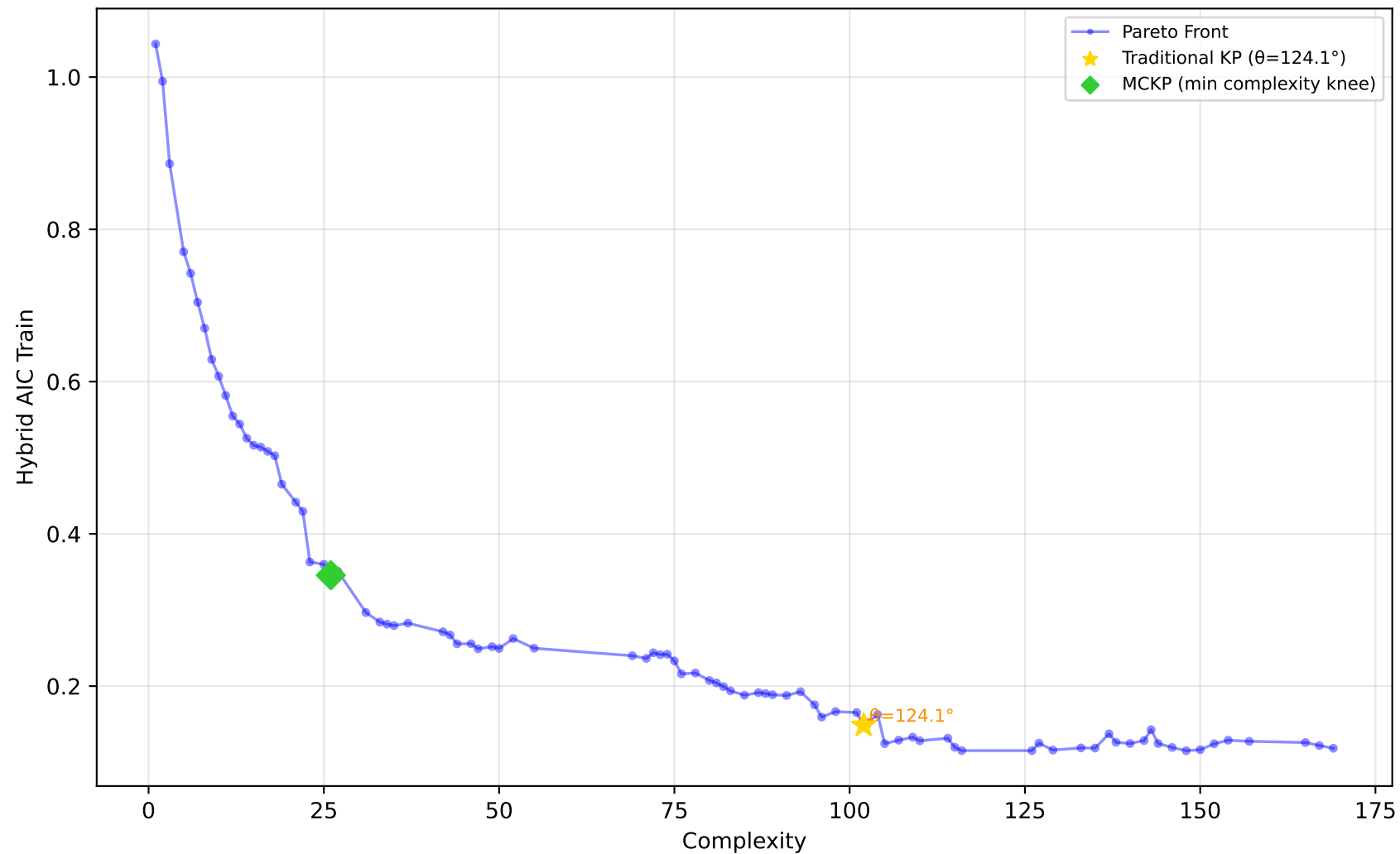
229_pwLinear - Run 22 - SVP - Hybrid AIC Train \lambda_1=0.50, \lambda_2=0.10, \lambda_3=0.00 | Difficulty: 1.00 | Method: hmr
