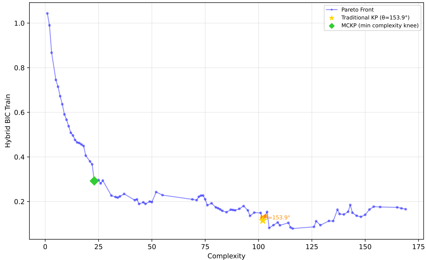
229_pwLinear - Run 22 - SVP - Hybrid BIC Train \lambda_1=0.50 , \lambda_2=0.00 , \lambda_3=0.00 | Difficulty: 1.00 | Method: hmr
