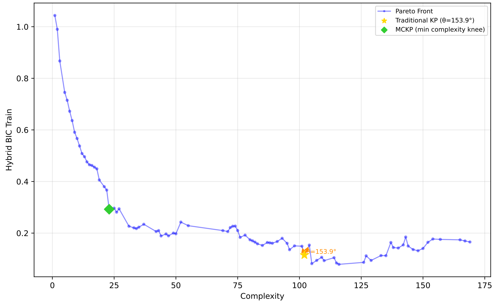
229_pwLinear - Run 22 - SVP - Hybrid BIC Train \lambda_1=0.50 , \lambda_2=0.10 , \lambda_3=0.00 | Difficulty: 1.00 | Method: hmr
