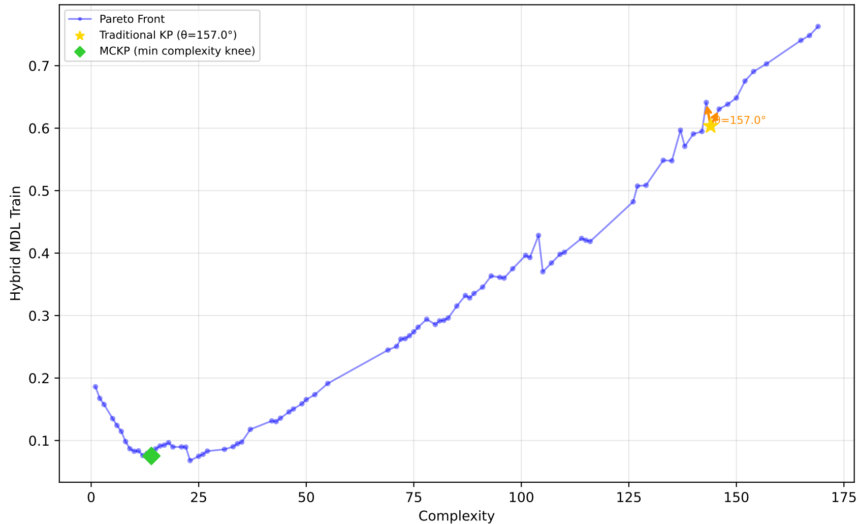
229_pwLinear - Run 22 - SVP - Hybrid MDL Train \lambda_1=0.50, \lambda_2=0.00, \lambda_3=0.00 | Difficulty: 1.00 | Method: hmr
