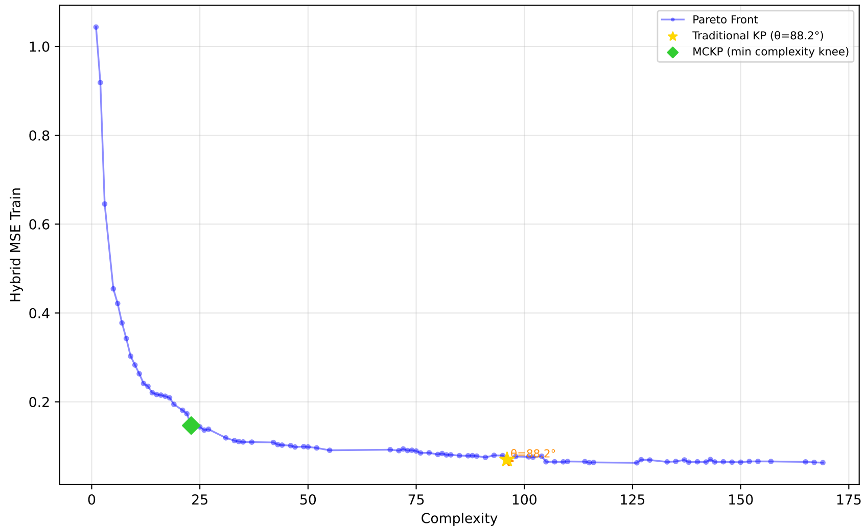
229_pwLinear - Run 22 - SVP - Hybrid MSE Train \lambda_1=0.50, \lambda_2=0.00, \lambda_3=0.00 | Difficulty: 1.00 | Method: hmr
