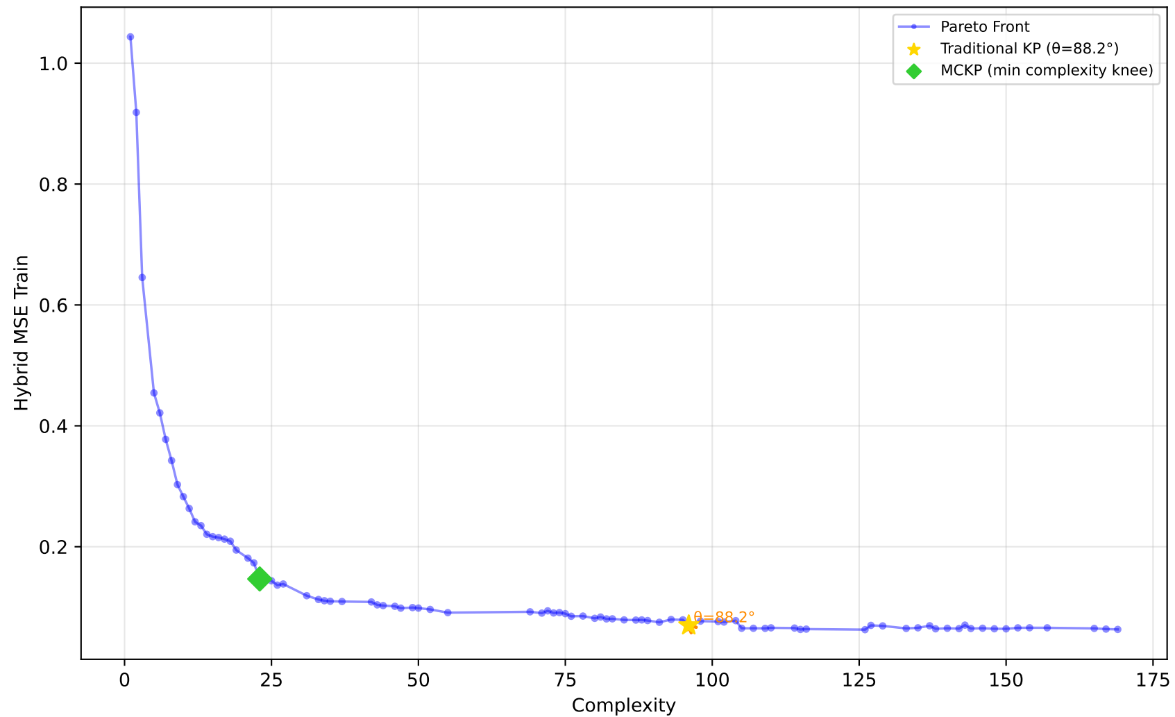
229_pwLinear - Run 22 - SVP - Hybrid MSE Train \lambda_1=0.50, \lambda_2=0.10, \lambda_3=0.00 | Difficulty: 1.00 | Method: hmr
