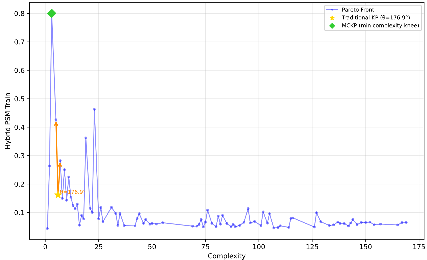
229_pwLinear - Run 22 - SVP - Hybrid PSM Train \lambda_1=0.50, \lambda_2=0.00, \lambda_3=0.00 | Difficulty: 1.00 | Method: hmr
