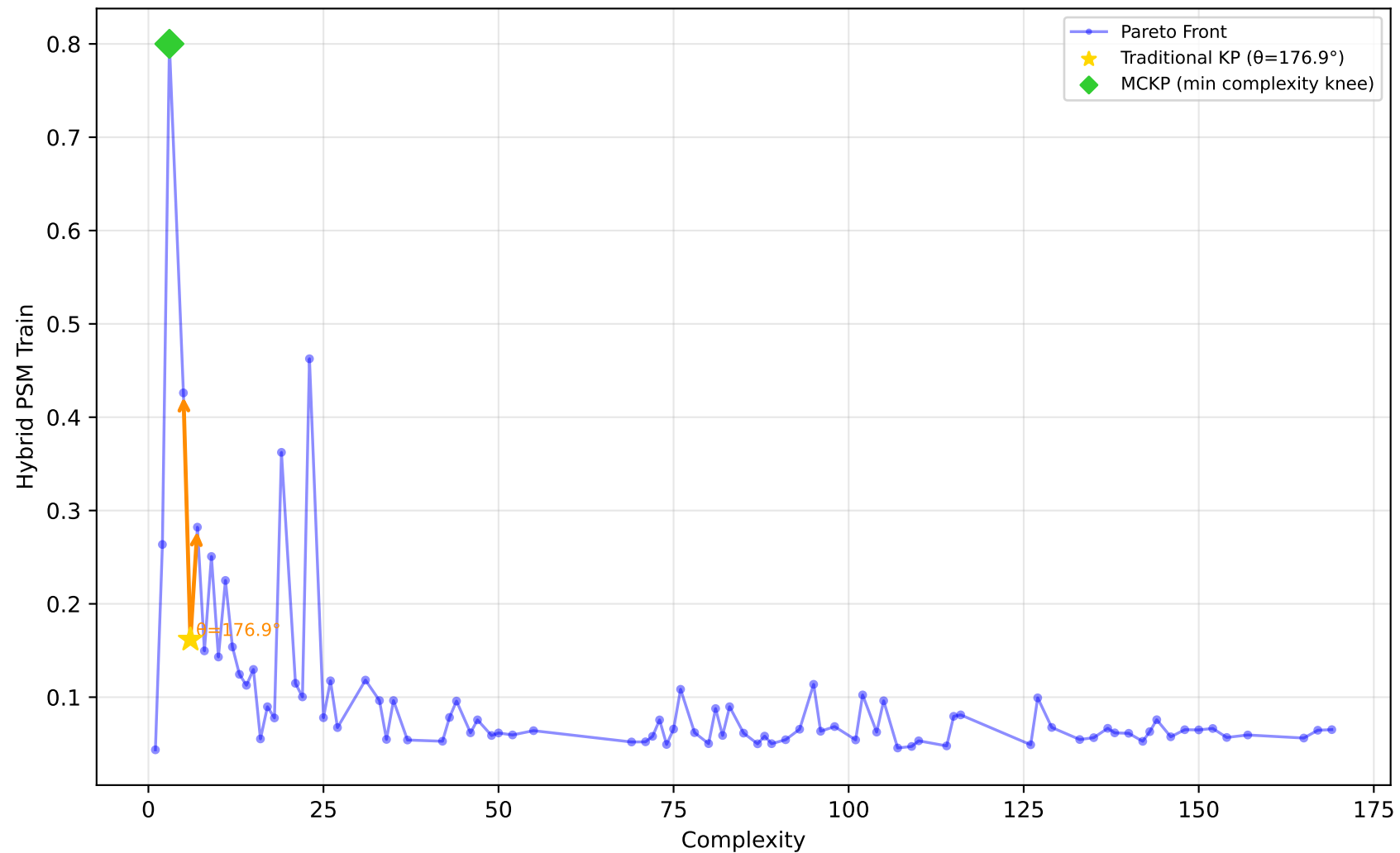
229_pwLinear - Run 22 - SVP - Hybrid PSM Train \lambda_1=0.50, \lambda_2=0.10, \lambda_3=0.00 | Difficulty: 1.00 | Method: hmr
