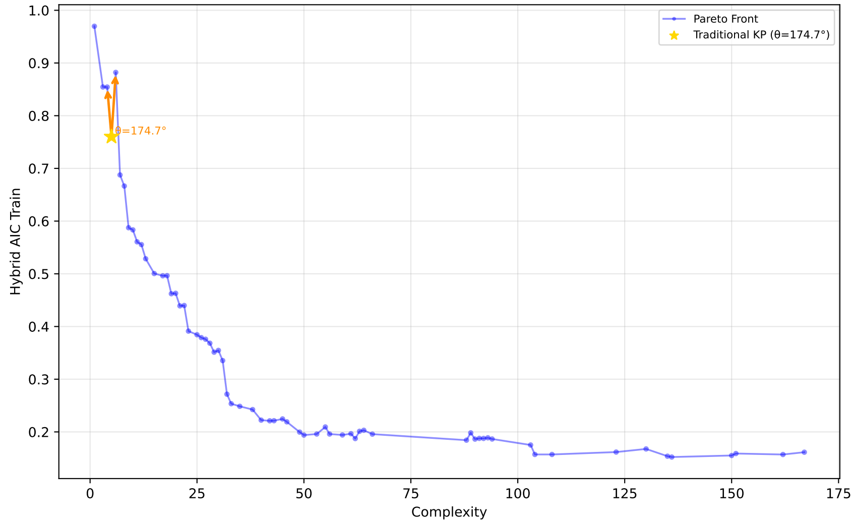
229_pwLinear - Run 23 - MVP - Hybrid AIC Train \lambda_1=0.50, \bar{\lambda}_2=0.00, \lambda_3=0.00 | Difficulty: 1.00 | Method: hmr
