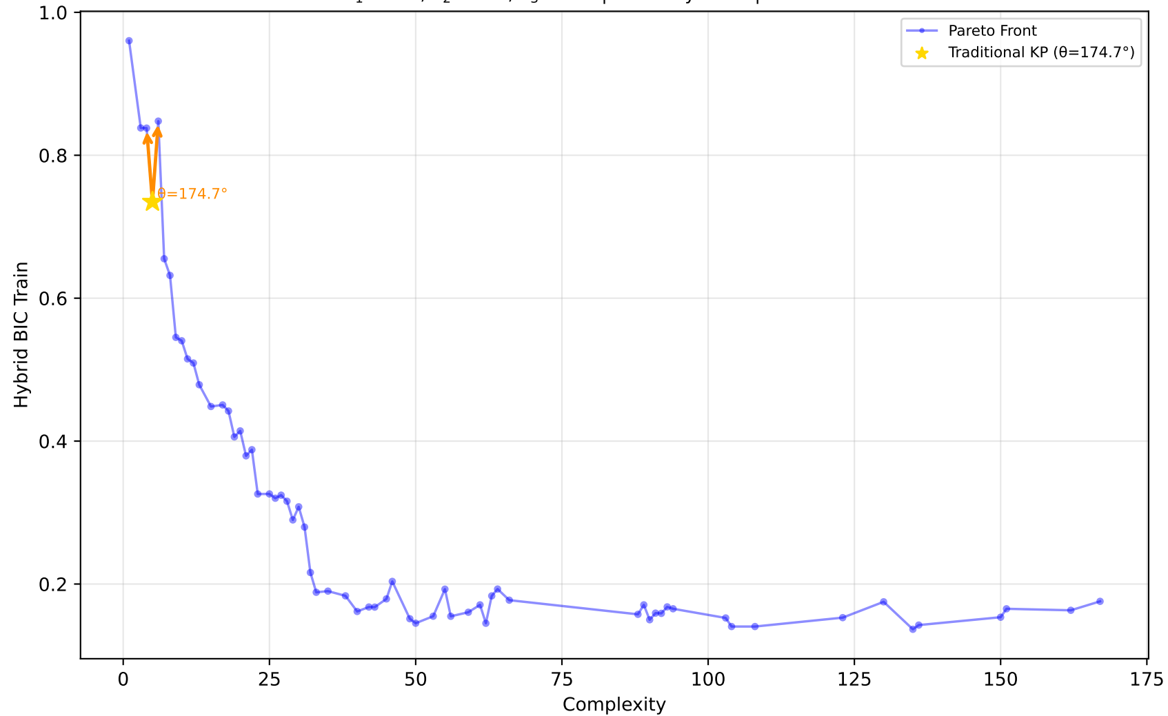
229_pwLinear - Run 23 - MVP - Hybrid BIC Train \lambda_1=0.50, \bar{\lambda}_2=0.00, \lambda_3=0.00 | Difficulty: 1.00 | Method: hmr
