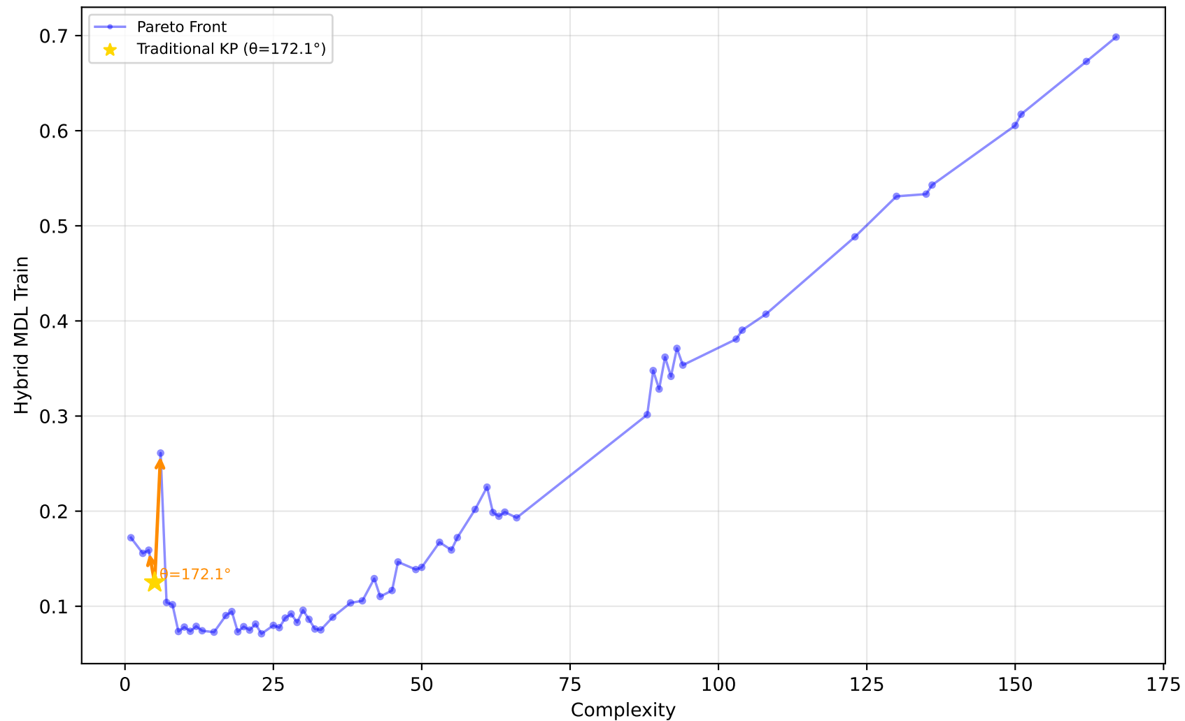
229_pwLinear - Run 23 - MVP - Hybrid MDL Train \lambda_1=0.50, \bar{\lambda}_2=0.00, \lambda_3=0.00 | Difficulty: 1.00 | Method: hmr
