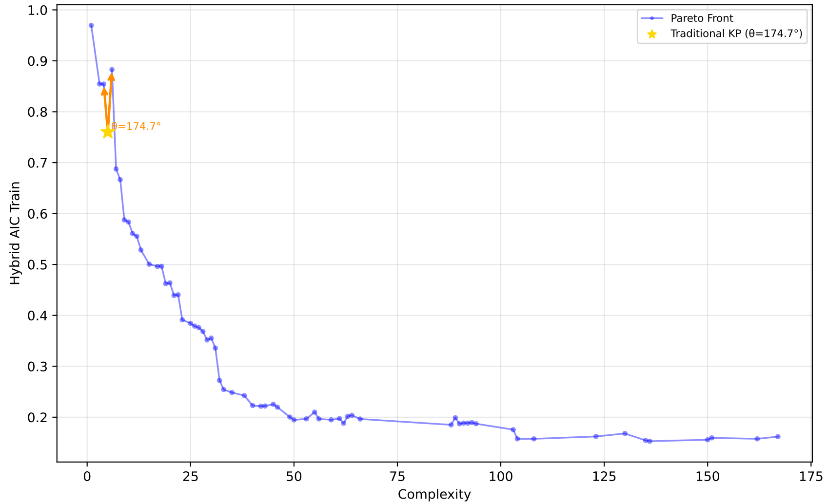
229_pwLinear - Run 23 - SVP - Hybrid AIC Train \lambda_1=0.50, \bar{\lambda}_2=0.10, \lambda_3=0.00 | Difficulty: 1.00 | Method: hmr
