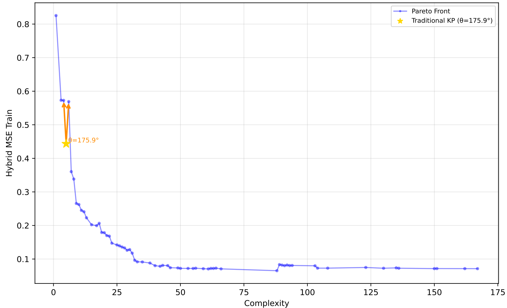
229_pwLinear - Run 23 - SVP - Hybrid MSE Train \lambda_1=0.50, \lambda_2=0.10, \lambda_3=0.00 | Difficulty: 1.00 | Method: hmr
