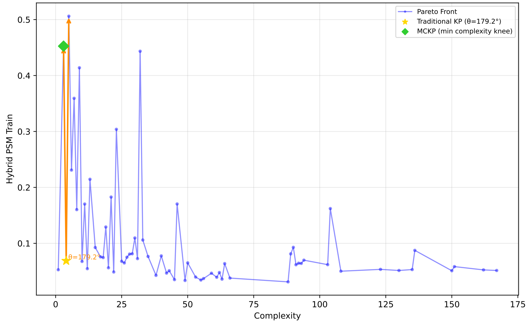
229_pwLinear - Run 23 - SVP - Hybrid PSM Train \lambda_1=0.50, \lambda_2=0.00, \lambda_3=0.00 | Difficulty: 1.00 | Method: hmr
