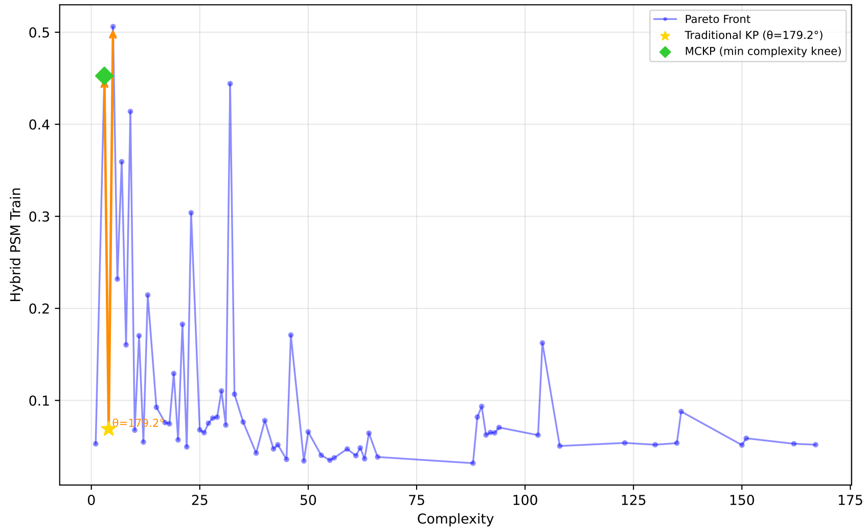
229_pwLinear - Run 23 - SVP - Hybrid PSM Train \lambda_1=0.50, \lambda_2=0.10, \lambda_3=0.00 | Difficulty: 1.00 | Method: hmr
