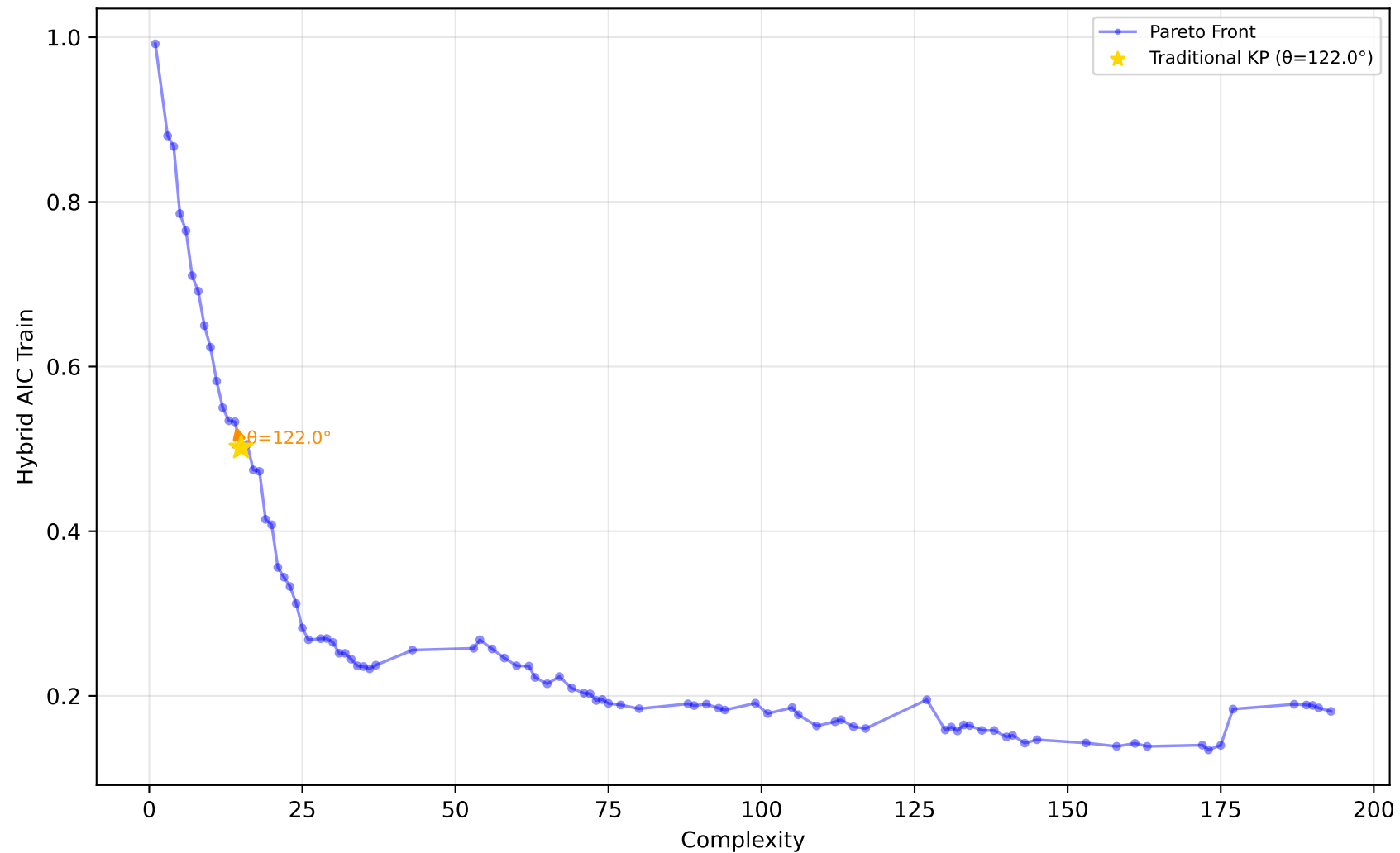
229_pwLinear - Run 24 - MVP - Hybrid AIC Train \lambda_1=0.50, \lambda_2=0.00, \lambda_3=0.00 | Difficulty: 1.00 | Method: hmr
