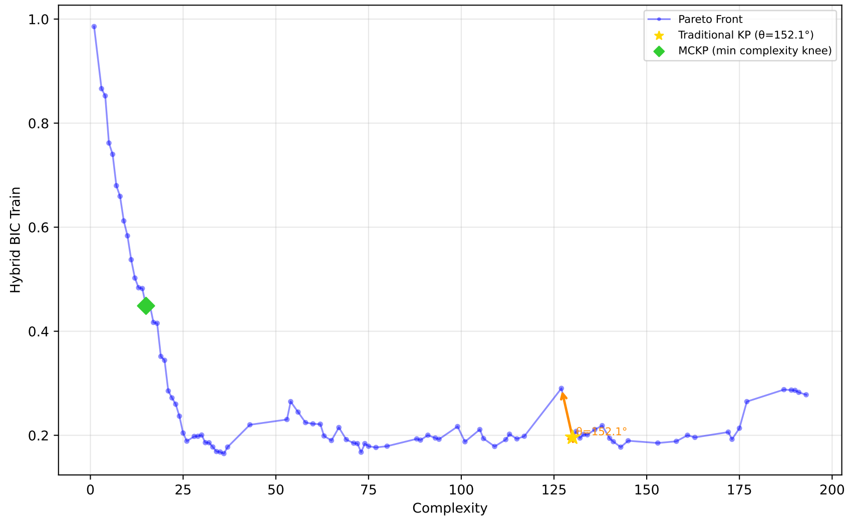
229_pwLinear - Run 24 - SVP - Hybrid BIC Train \lambda_1=0.50, \lambda_2=0.10, \lambda_3=0.00 | Difficulty: 1.00 | Method: hmr
