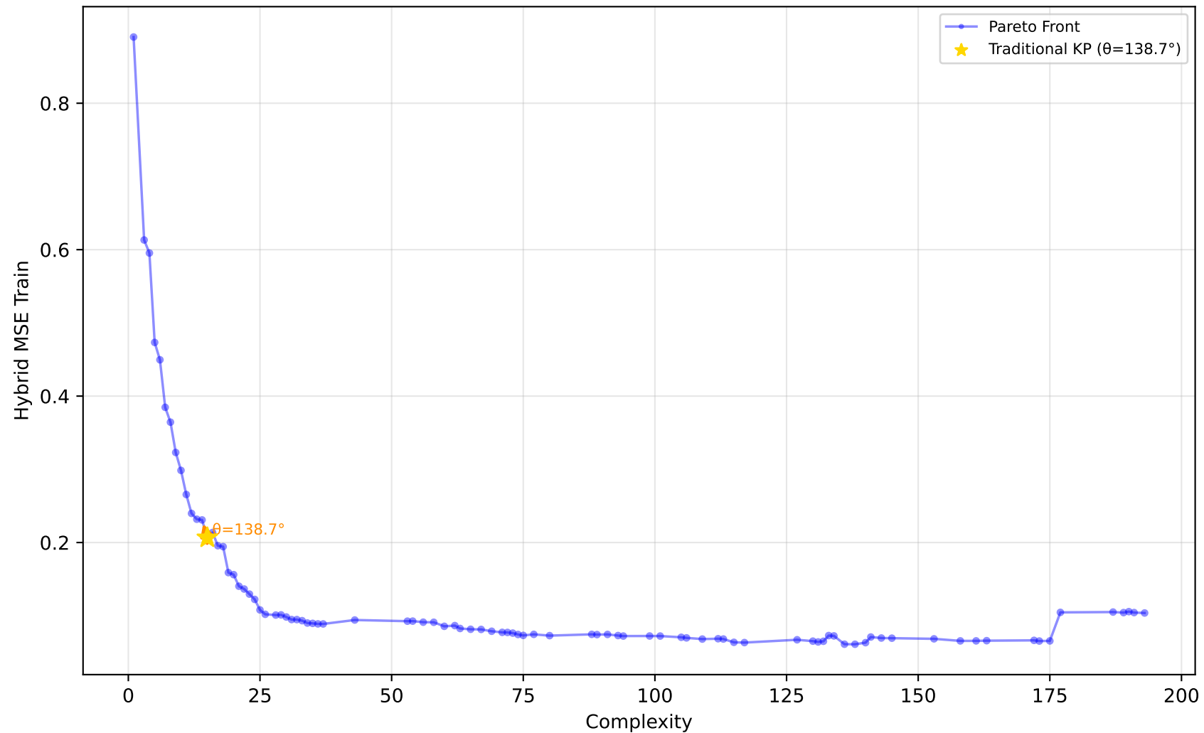
229_pwLinear - Run 24 - SVP - Hybrid MSE Train \lambda_1=0.50, \lambda_2=0.10, \lambda_3=0.00 | Difficulty: 1.00 | Method: hmr
