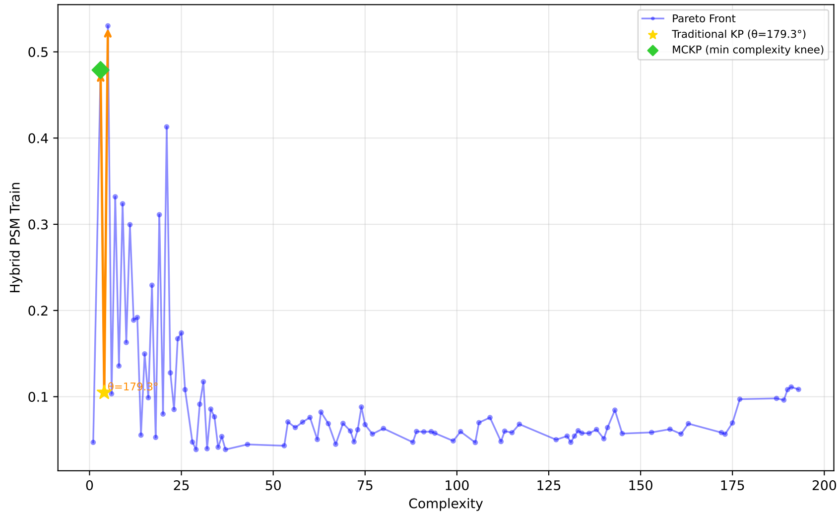
229_pwLinear - Run 24 - SVP - Hybrid PSM Train \lambda_1=0.50, \lambda_2=0.10, \lambda_3=0.00 | Difficulty: 1.00 | Method: hmr
