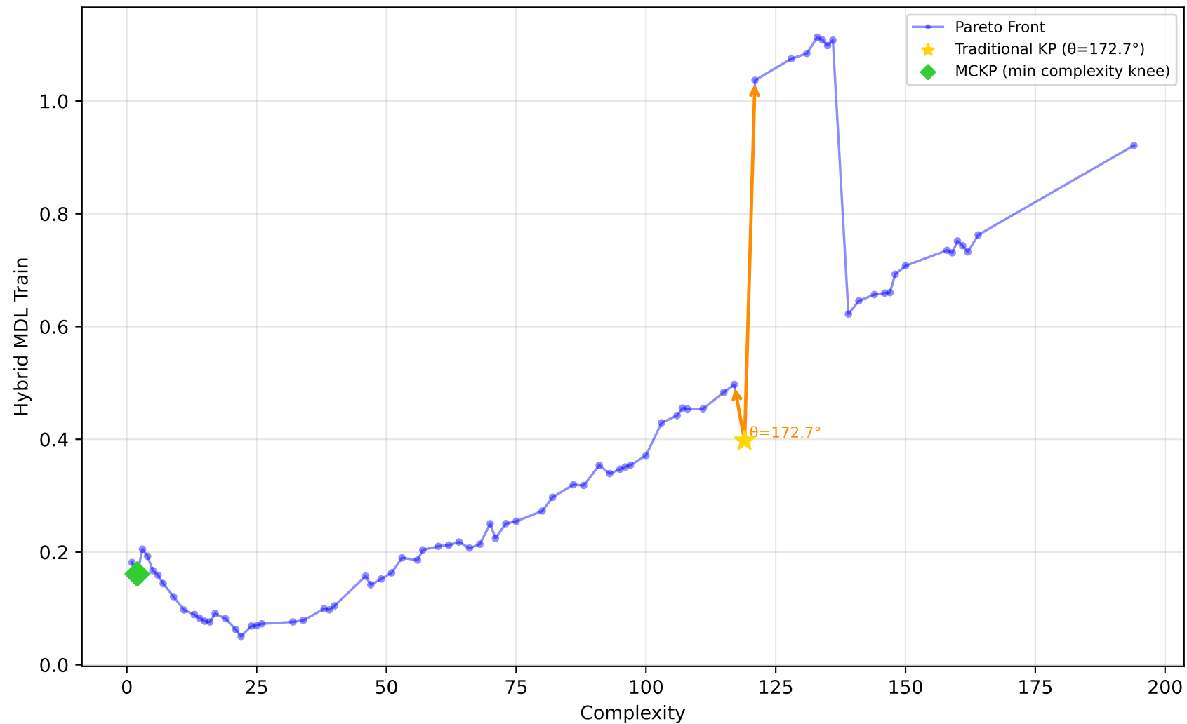
229_pwLinear - Run 25 - MVP - Hybrid MDL Train \lambda_1=0.50, \lambda_2=0.00, \lambda_3=0.00 | Difficulty: 1.00 | Method: hmr
