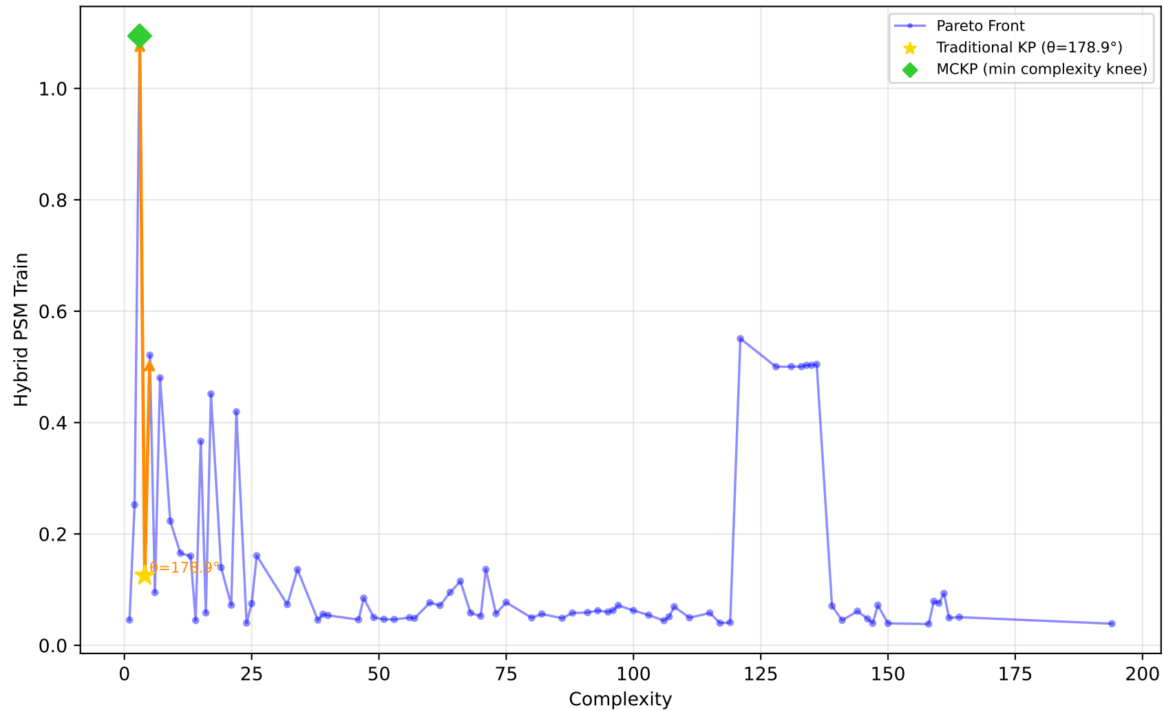
229_pwLinear - Run 25 - MVP - Hybrid PSM Train \lambda_1=0.50, \lambda_2=0.00, \lambda_3=0.00 | Difficulty: 1.00 | Method: hmr
