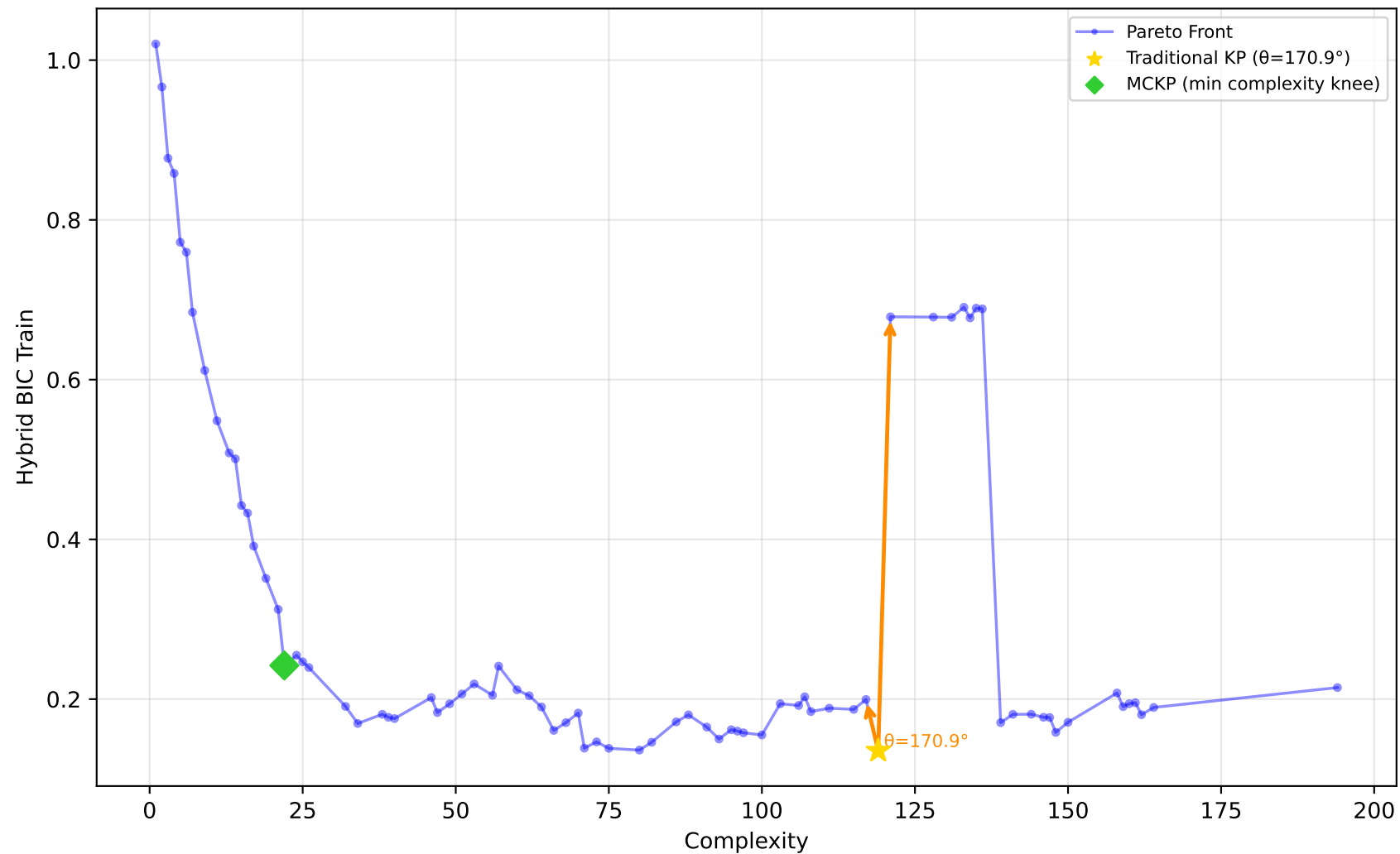
229_pwLinear - Run 25 - SVP - Hybrid BIC Train \lambda_1=0.50, \bar{\lambda}_2=0.00, \lambda_3=0.00 | Difficulty: 1.00 | Method: hmr
