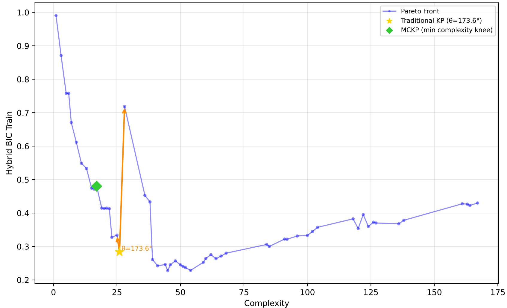
229_pwLinear - Run 26 - MVP - Hybrid BIC Train \lambda_1=0.50, \bar{\lambda}_2=0.00, \lambda_3=0.00 | Difficulty: 1.00 | Method: hmr
